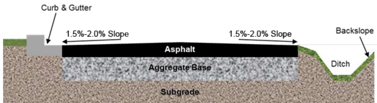
Figure 1.1. Schematic of surface drainage off a pavement surface into a roadside drainage ditch or curb and gutter (not to scale).
