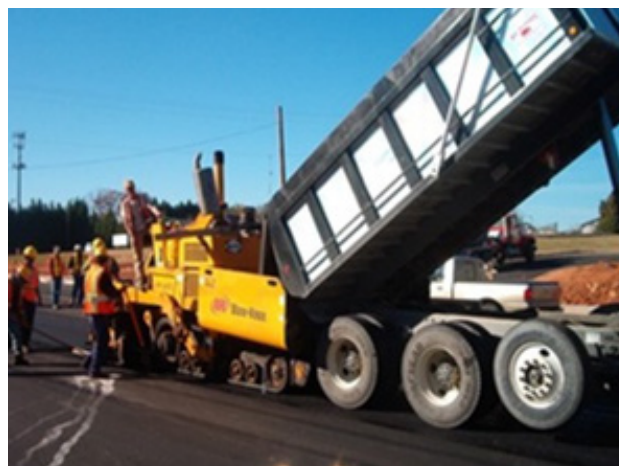
Haul truck depositing asphalt into a paver.
