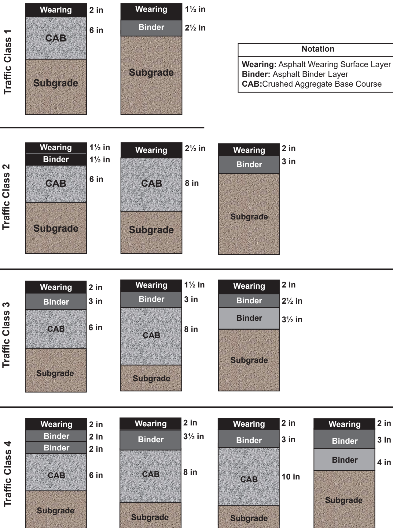
Figure 1.7. Recommended asphalt pavement thickness design options for different traffic classes on a Good Subgrade.
