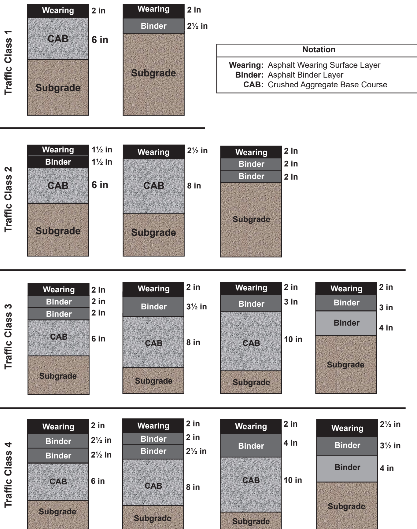
Figure 1.6. Recommended asphalt pavement thickness design options for different traffic classes on a Medium Subgrade.
