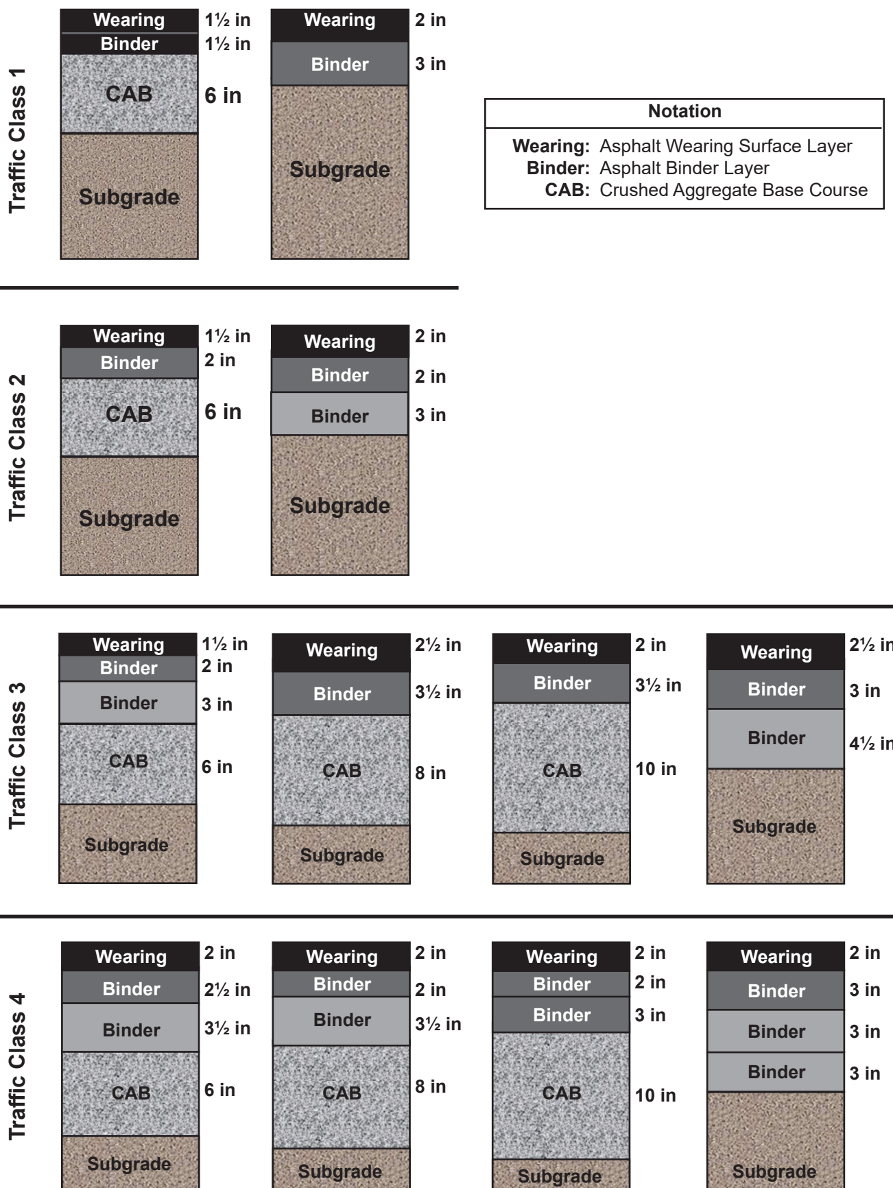
Figure 1.5. Recommended asphalt pavement thickness design options for different traffic classes on a Poor Subgrade.
