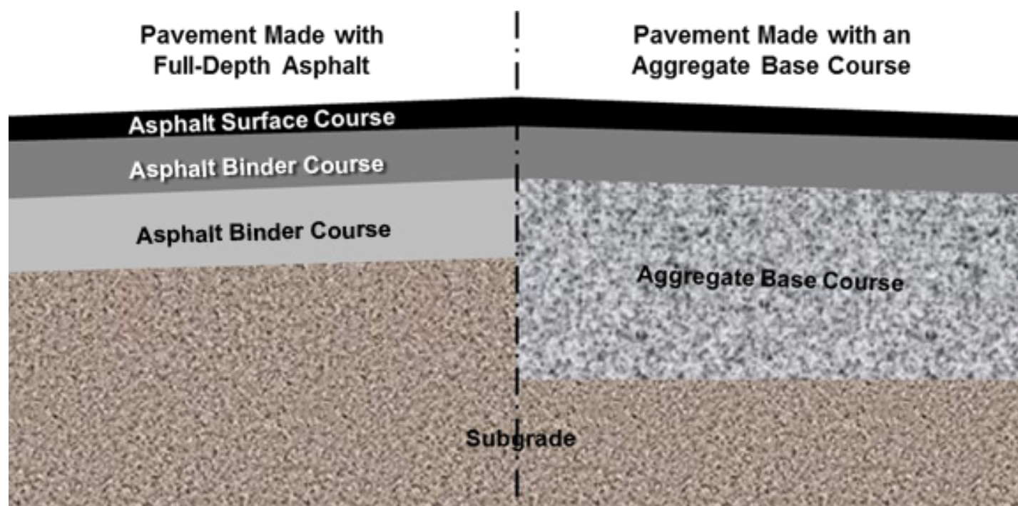
Figure 1.3. Typical cross-sections for full-depth asphalt pavements (on left) and asphalt pavements designed with an aggregate base course (on right) (not to scale).
