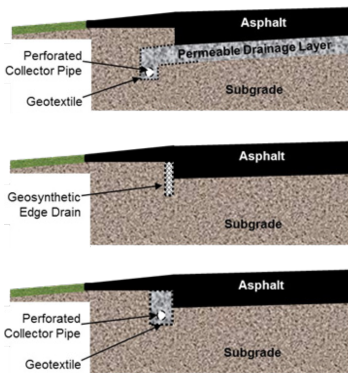
Figure 1.2. Schematics of typical subsurface drainage solutions (not to scale).
